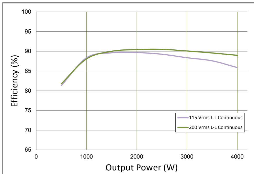
Figure 4: Efficiency vs Output Power
