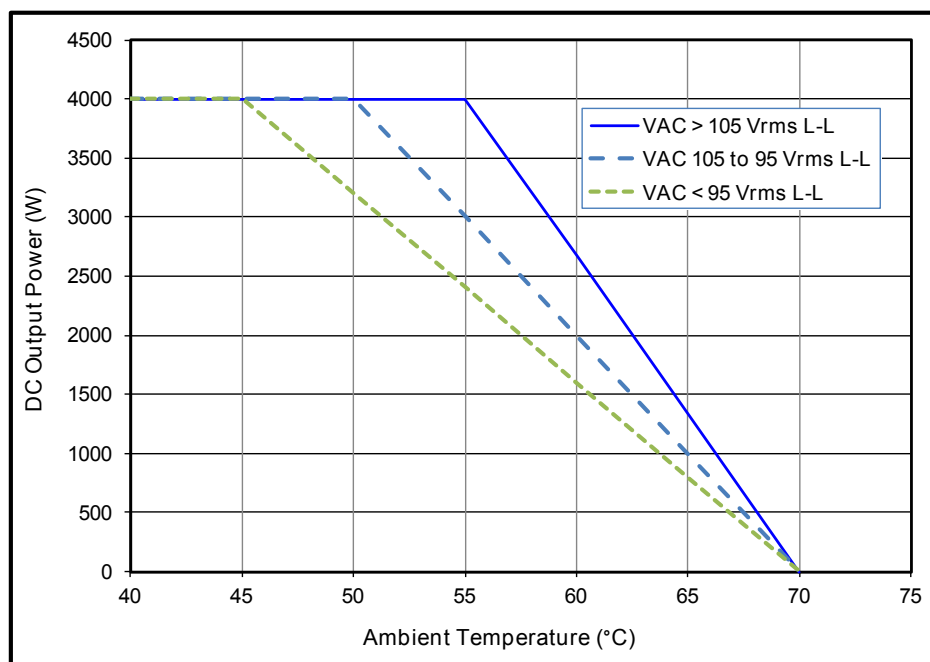
Figure 3: Output Power vs. Ambient Temperature
