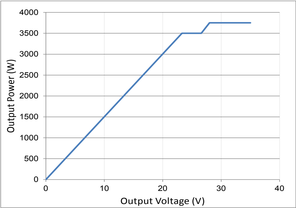
Figure 7: Vout derating. 28V model Available Output power vs Output voltagee
