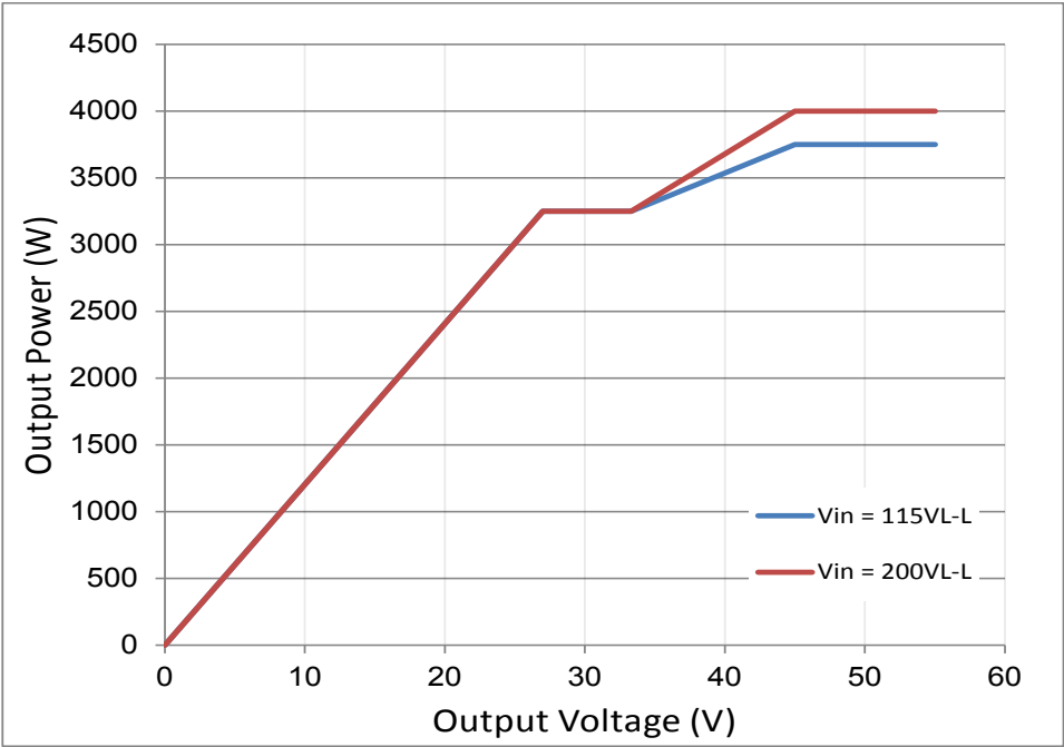
Figure 6: Vout derating. 48V model Available Output power vs Output voltagee
